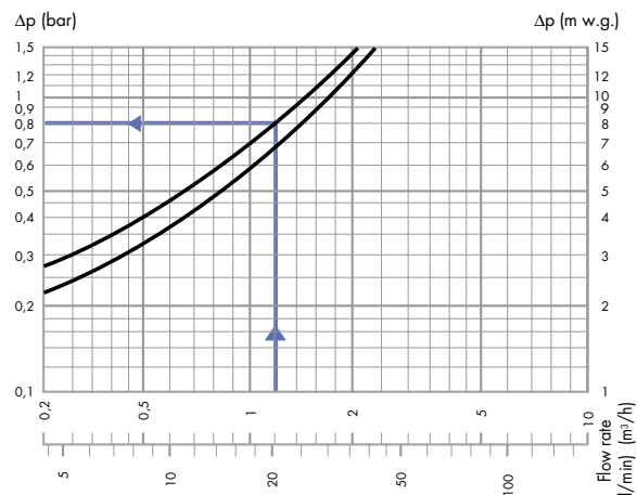
Diagram 2 (Pressure drop)
